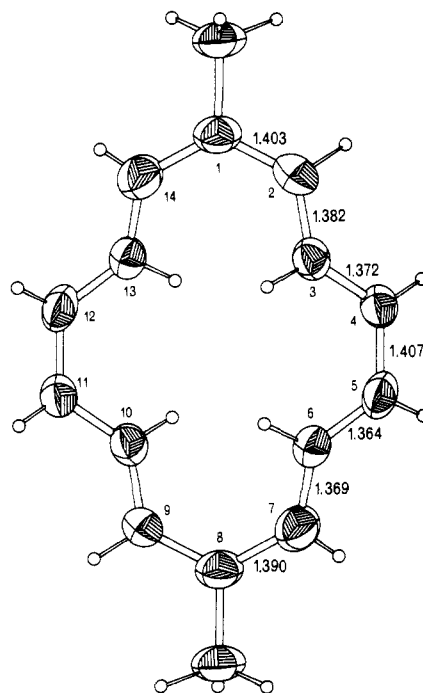
Figure 1. Molecular structure of 1,8-dimethyl[14]annulene ( 5a ).
